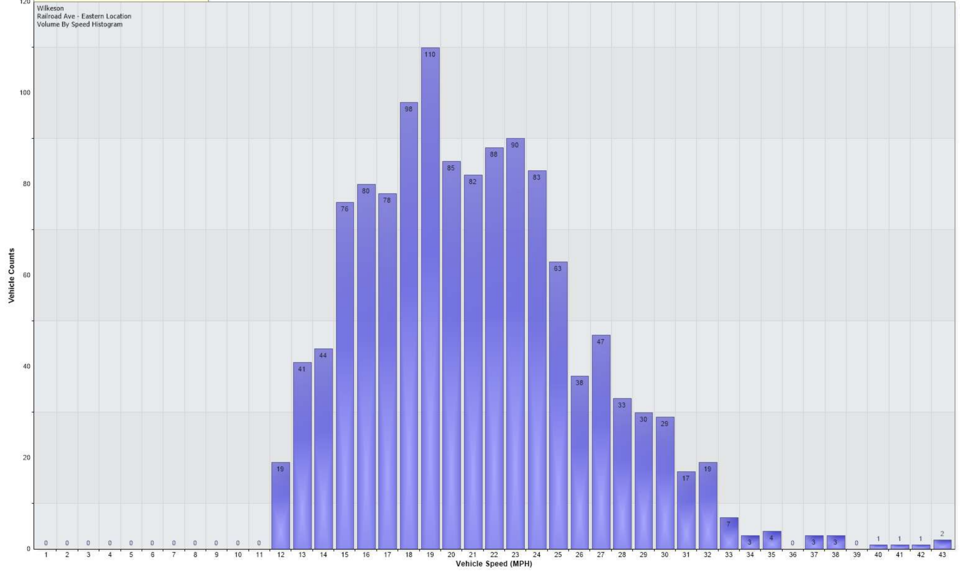
Vehicle Counts Vs. Speed [Wilkeson: Westbound]
