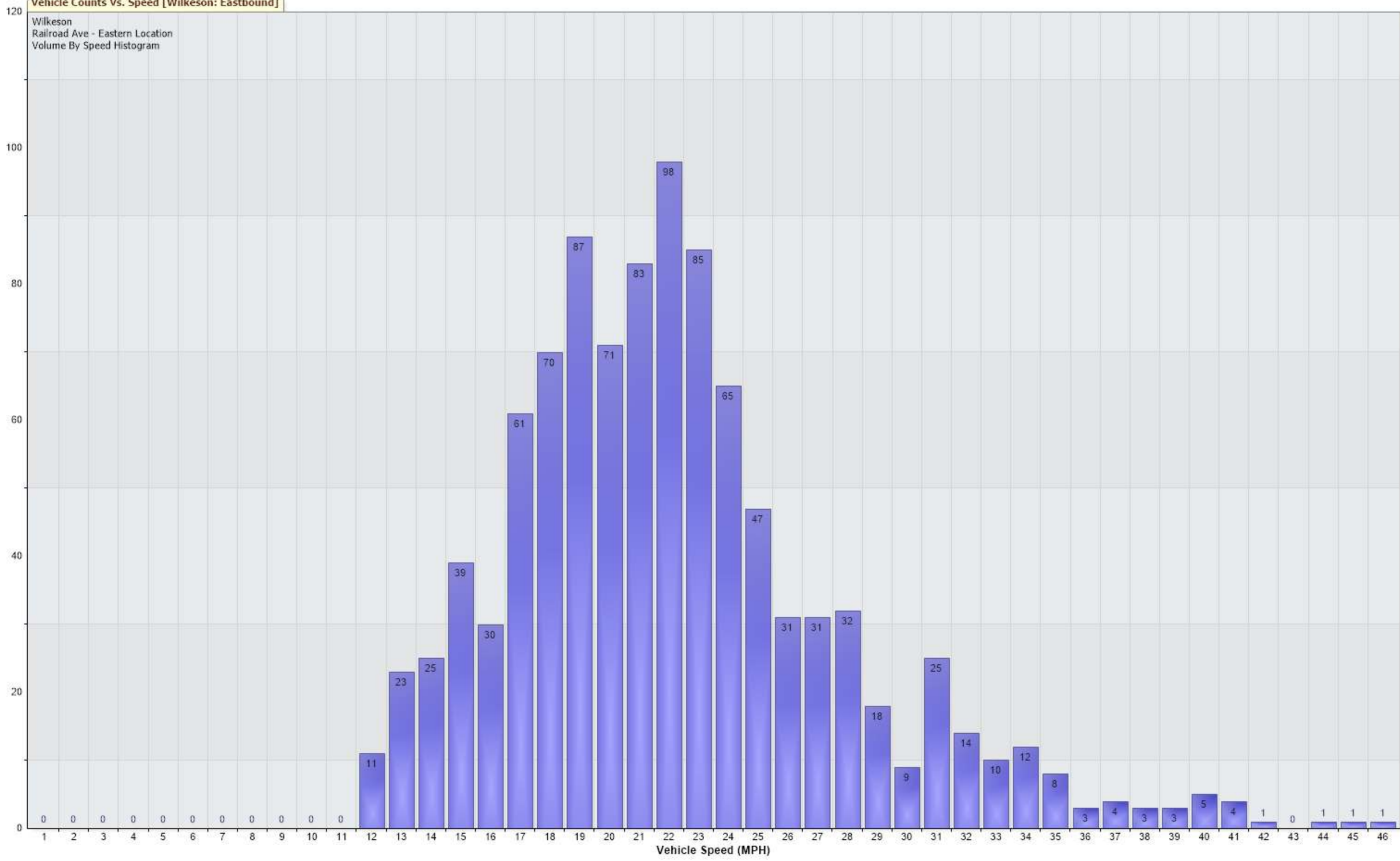
Vehicle Counts Vs. Speed [Wilkeson: Eastbound]
